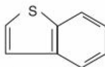
Benzothiophene
