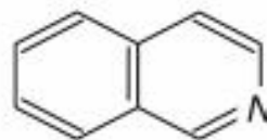
isoquinoline ( C_9H_7N )
