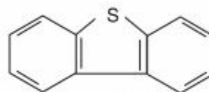
Dibenzothiophene
