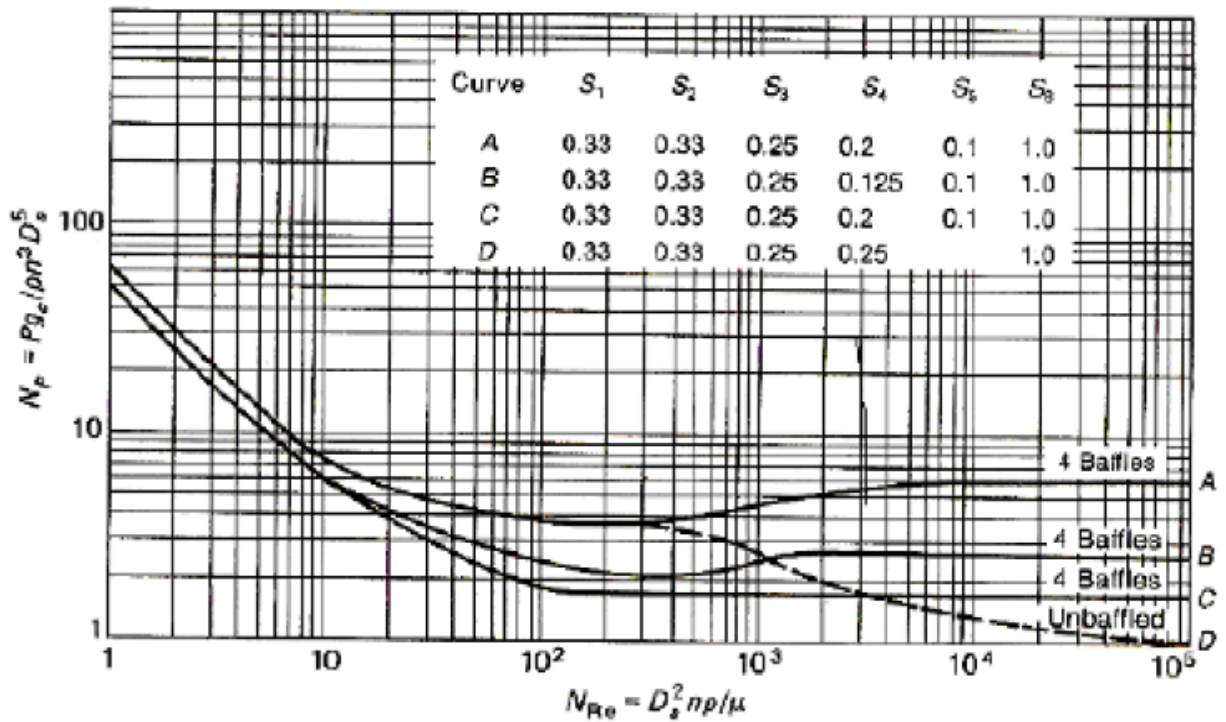
Power number N_p versus N_{Re} for six-blade turbines. With the dashed portion of curve D, the value of N_p read from the figure must be multiplied by N_{Re}^m .
