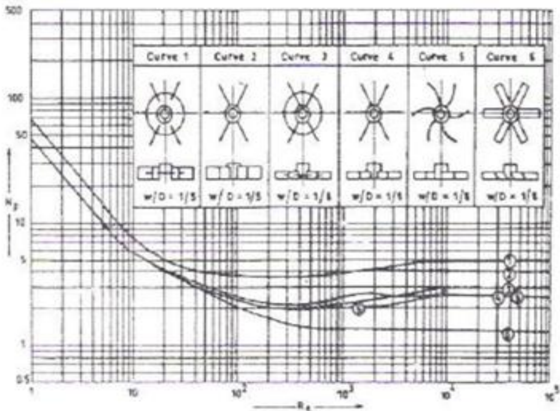
Power correlation for a 6 – blade turbine in pseudo plastic liquids
