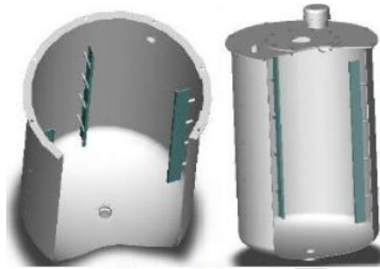
Figure : Baffled vessel.
